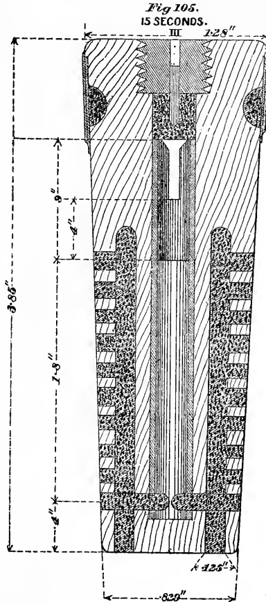
Boxes 15-seconds time-fuze.
